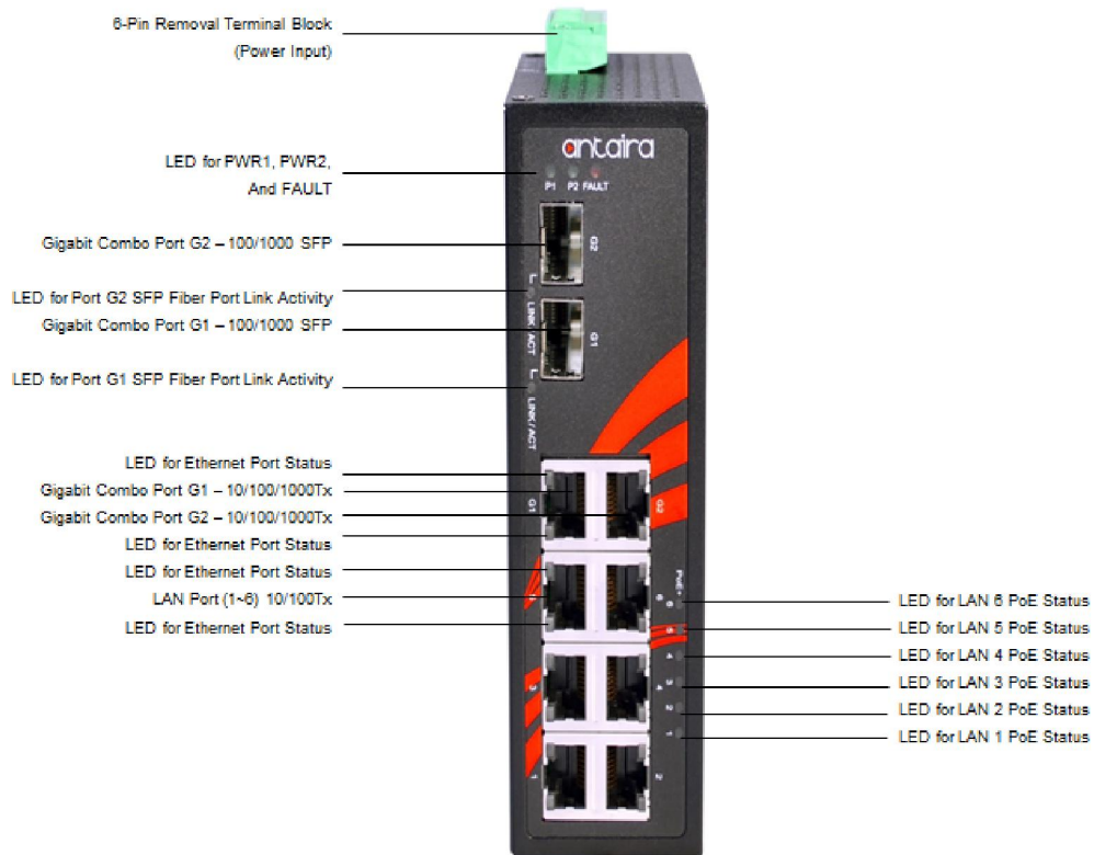
Figure 2.2 - The Front Panel of the LNP-0802C-SFP Series
